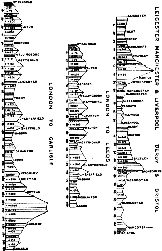
Fig. 86.—Section showing Gradients of Midland Railway.
